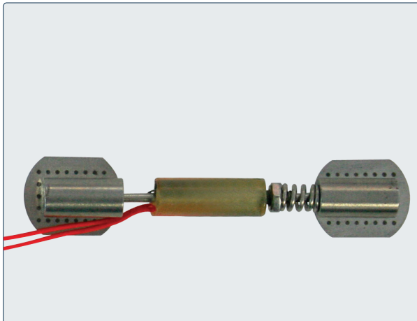
Vibrating Wire Spot Weldable Strain Gauge - Low Profile (VWSG-S-3000 or VWSG-S-5000)
